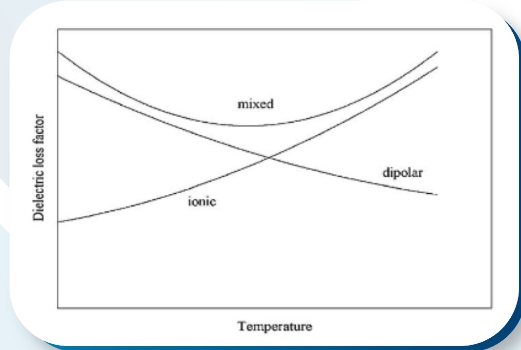
Variation of loss factor components with temperature
