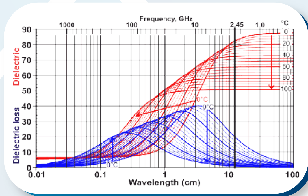
Dielectric loss water
